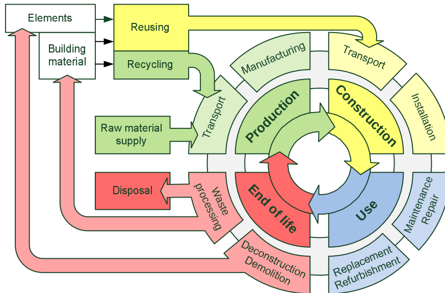
Figure 1. Structural elements life cycle
