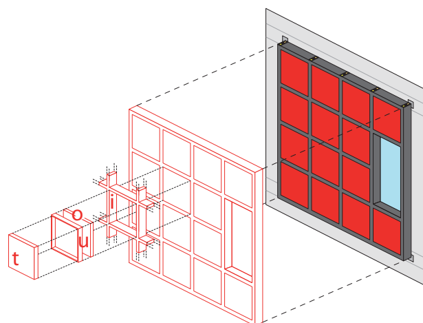
t Technological unit u Structural module i Structural panel o Thermal Insulation t + u Technological module t + u + i Multifunctional panel
