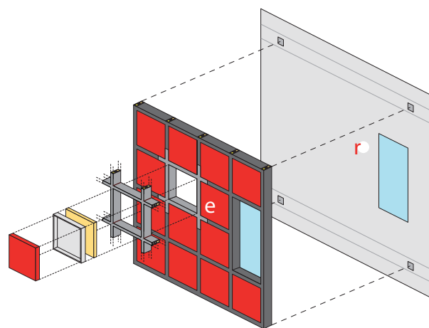
e Multifunctional panel r Existing facade
